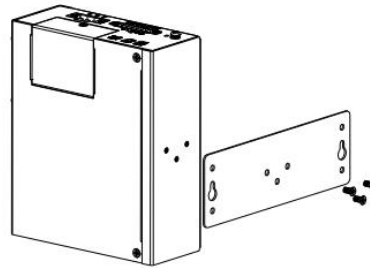
Wall mounting
