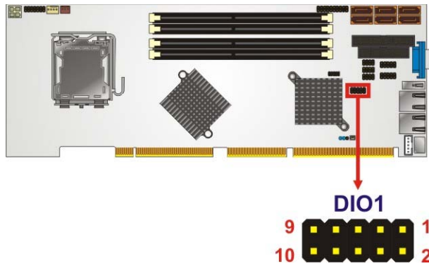
Figure 4-5: DIO Connector Location
