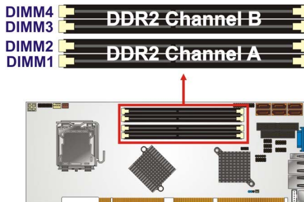
Figure 5-7: DDR2 Channels
