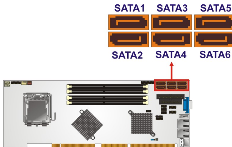
Figure 4-12: SATA Drive Connector Locations
