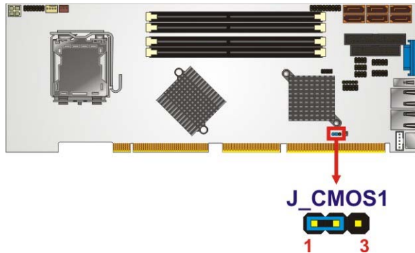
Figure 5-9: Clear CMOS Jumper
