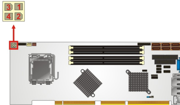
Figure 4-4: CPU Power Connector Location
