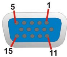
Figure 4-20: VGA Connector
