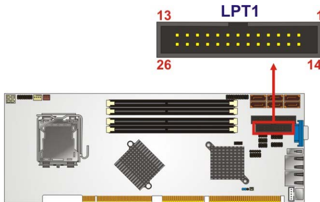
Figure 4-11: Parallel Port Connector Location
