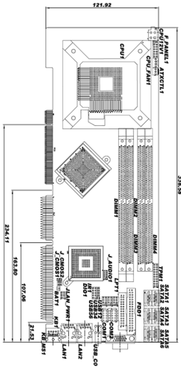
Figure 2-1: WSB-Q354 Dimensions (mm)
