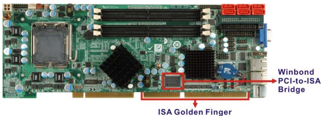
Figure 2-11: PCI-to-ISA Bridge and ISA Slot Connector
