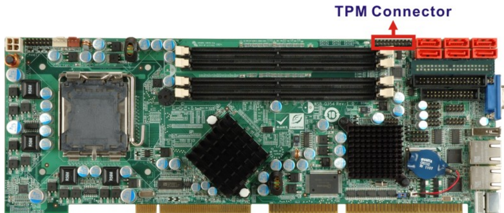
Figure 2-12: TPM Connector
