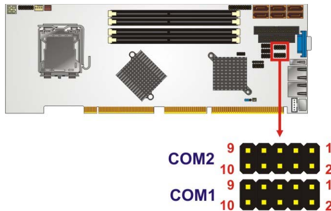
Figure 4-13: Serial Connector Location
