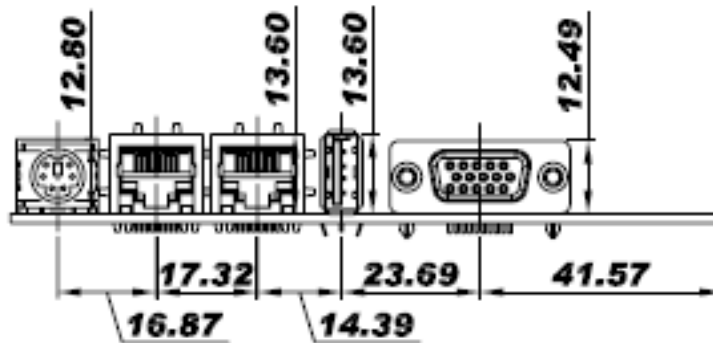
Figure 2-2: External Interface Panel Dimensions (mm)
