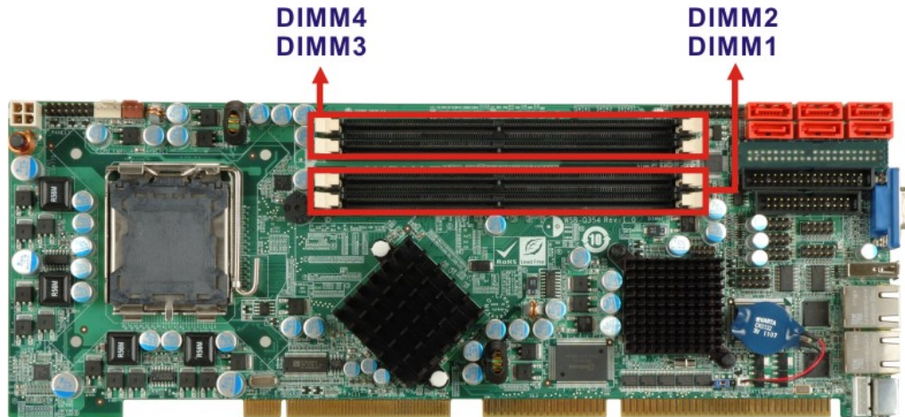
Figure 2-5: DDR2 DIMM Sockets
