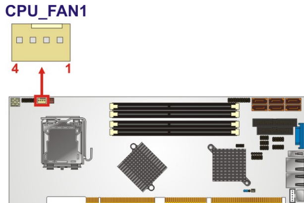
Figure 4-6: +12V Fan Connector Location
