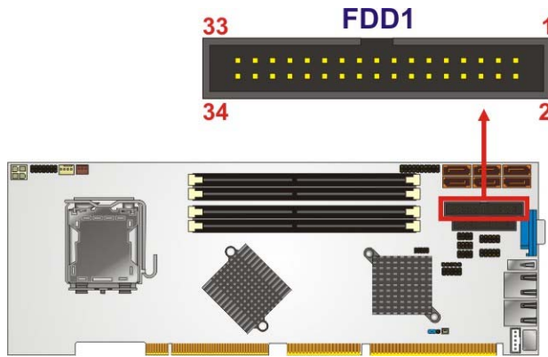
Figure 4-7: 34-pin FDD Connector Location
