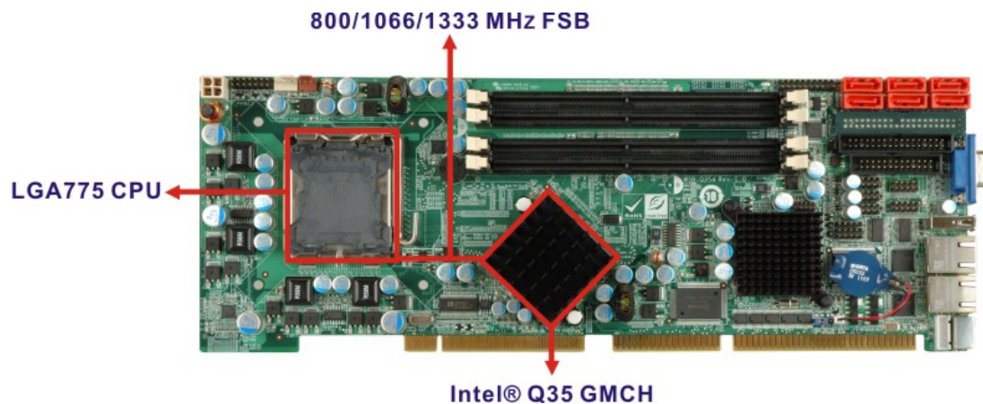
Figure 2-4: Front Side Bus (FSB)
