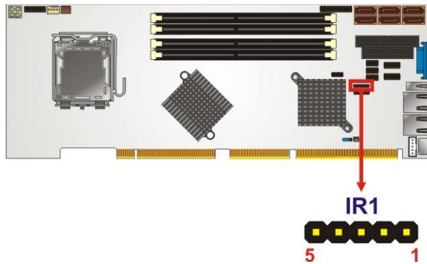
Figure 4-9: Infrared Connector Location
