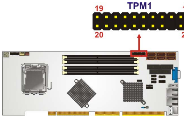
Figure 4-15: TPM Connector Location
