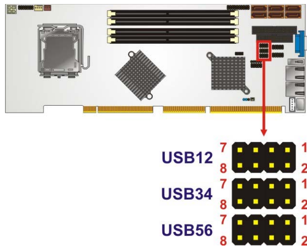
Figure 4-16: USB Connector Locations
