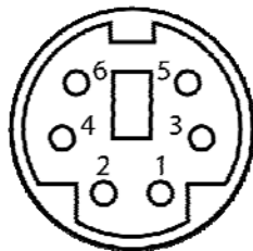
Figure 4-18: PS/2 Pinouts
