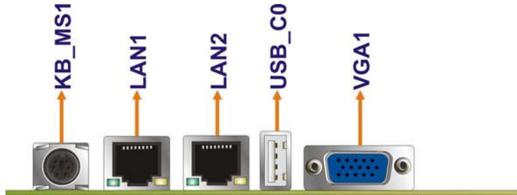
Figure 4-17: WSB-Q354 External Peripheral Interface Connector
