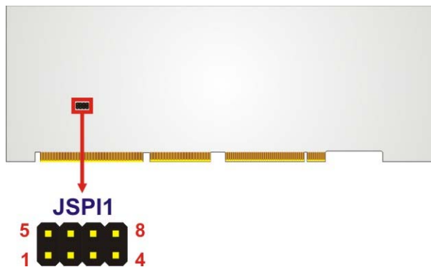
Figure 4-14: SPI Flash Connector Location (Solder Side)
