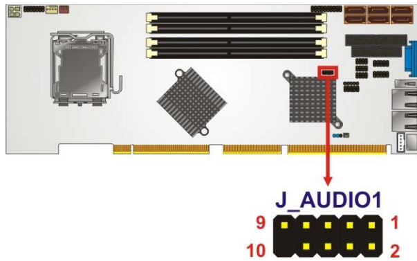
Figure 4-2: Audio Connector Pinouts (4-pin)
