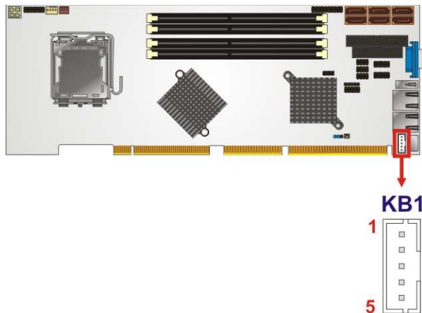
Figure 4-10: Keyboard Connector Location
