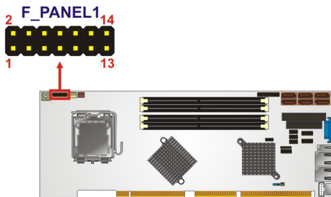
Figure 4-8: Front Panel Connector Pinout Locations (14-pin)
