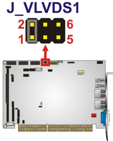
Figure 4-6: LVDS Voltage Selection Jumper Pinout Locations
