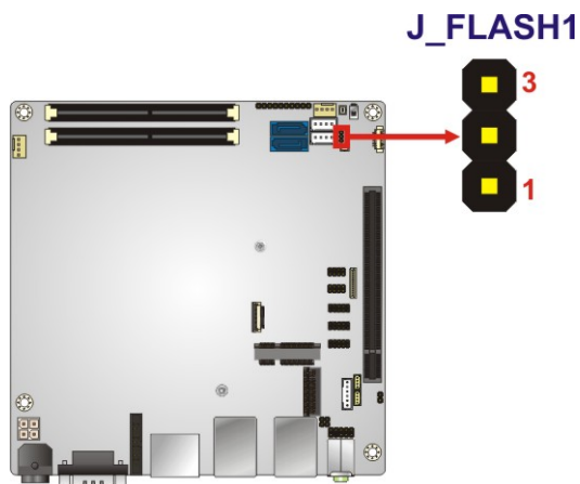
Figure 4-14: Flash Descriptor Security Override Jumper Location
