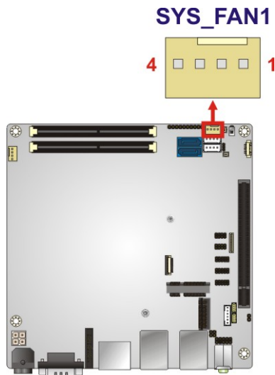
Figure 3-11: System Fan Connector Location
