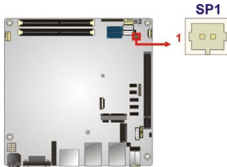
Figure 3-5: Buzzer Connector Location
