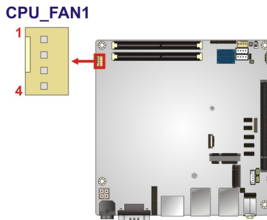
Figure 3-10: CPU Fan Connector Location
