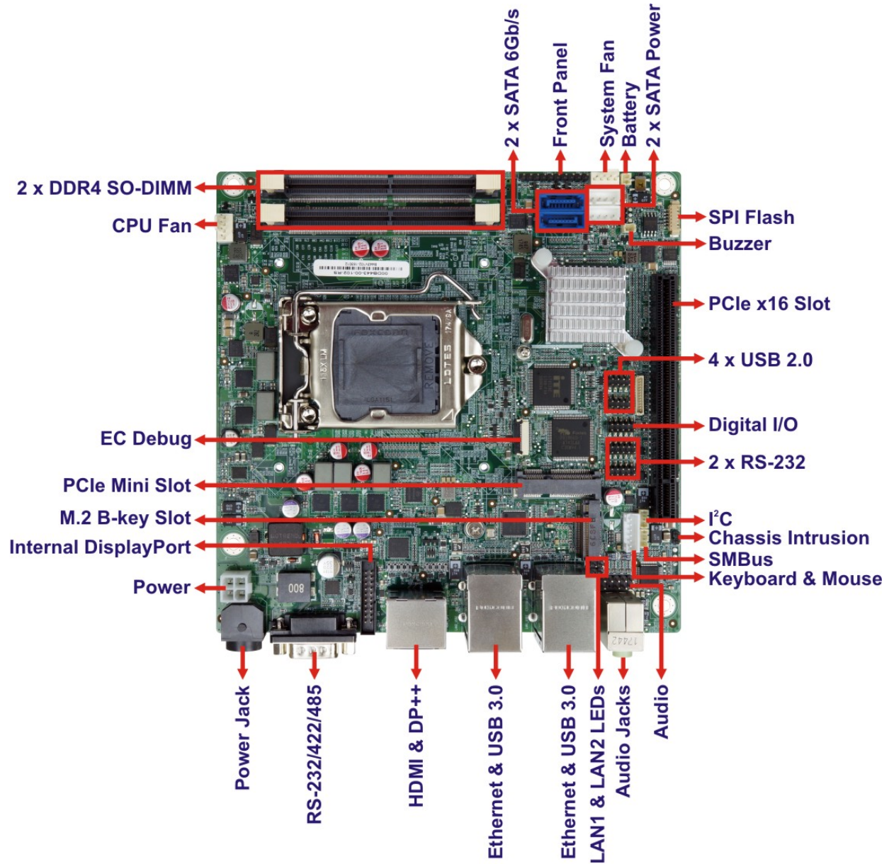
Figure 1-2: Connectors
