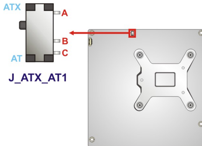
Figure 4-12: AT/ATX Power Mode Switch Location
