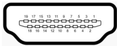
Figure 3-31: HDMI Connector
