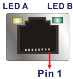
Figure 3-33: Ethernet Connector
