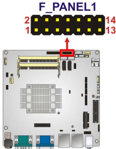
Figure 3-10: Front Panel Connector Location
