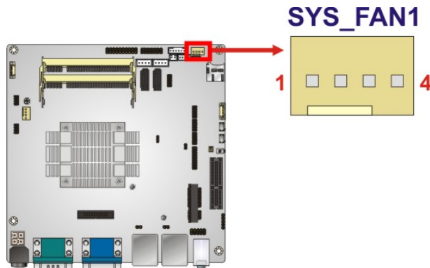
Figure 3-9: System Fan Connector Location
