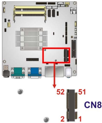
Figure 3-15: PCIe Mini Card Slot Location
