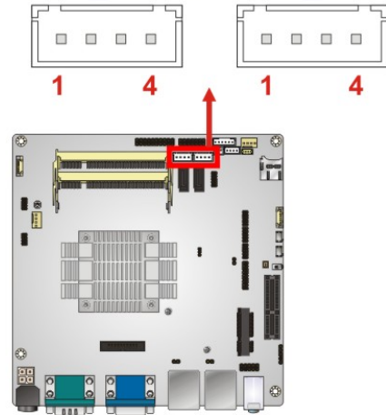
Figure 3-20: SATA Power Connector Locations
