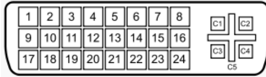
Figure 3-31: DVI-I Connector
