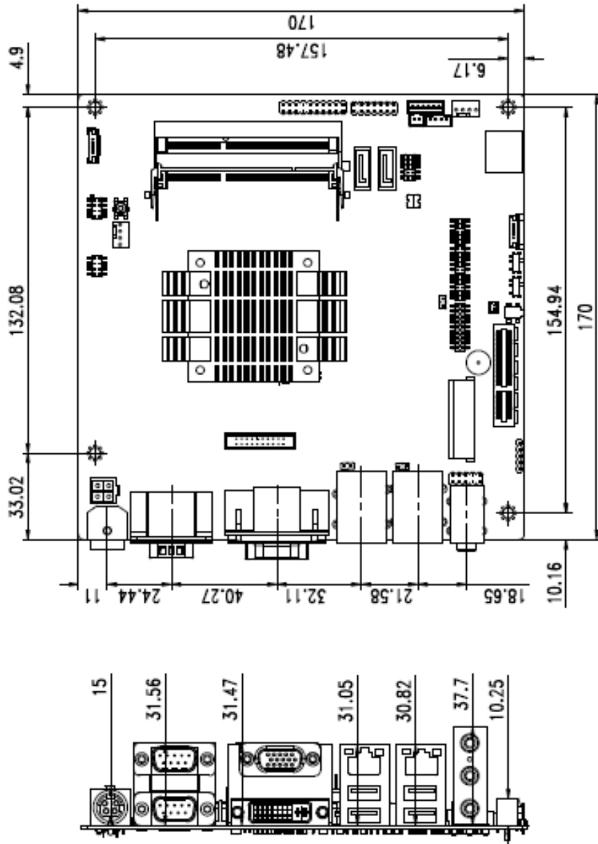
Figure 1-3: KINO-DBT Series Main Dimensions (mm)
