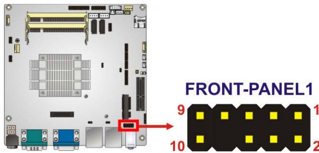
Figure 3-2: Audio Connector Location
