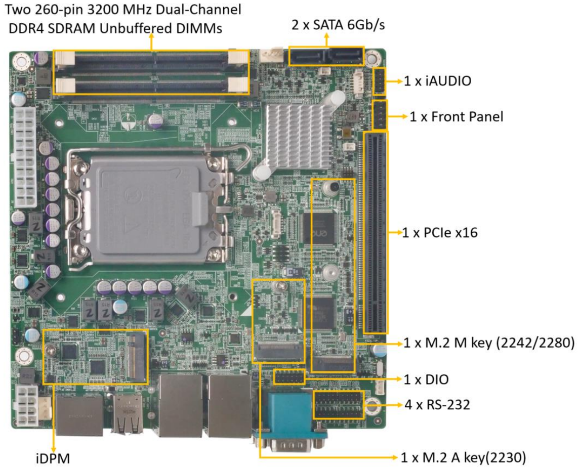
Figure 1-2: Connectors
