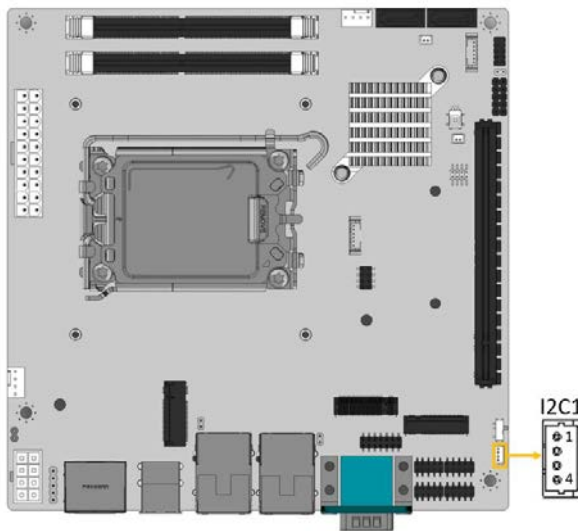
Figure 3-10: I 2 C/SMBus Connector Location
