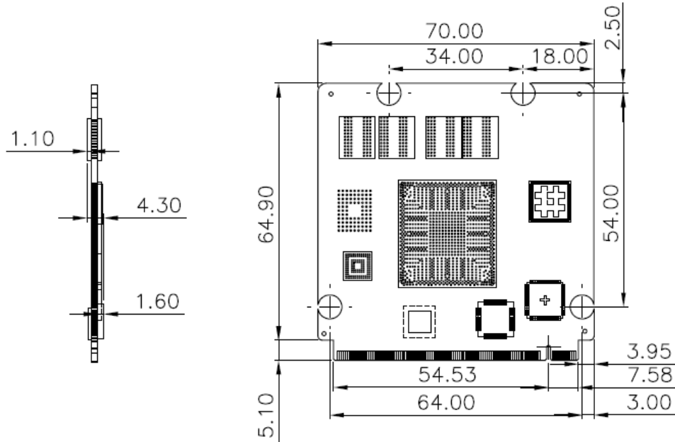
Figure 1-3: iQ7-BT Dimensions (mm)
