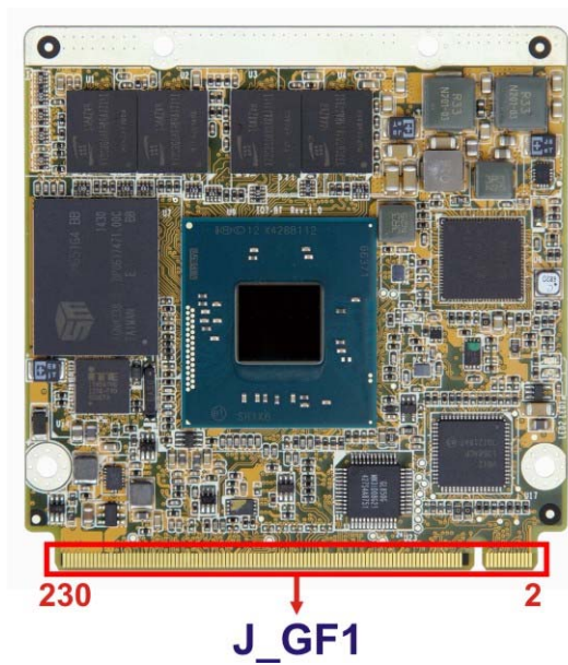
Figure 3-1: Qseven Connector Location
