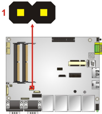
Figure 4-2: ME Override Jumper Location
