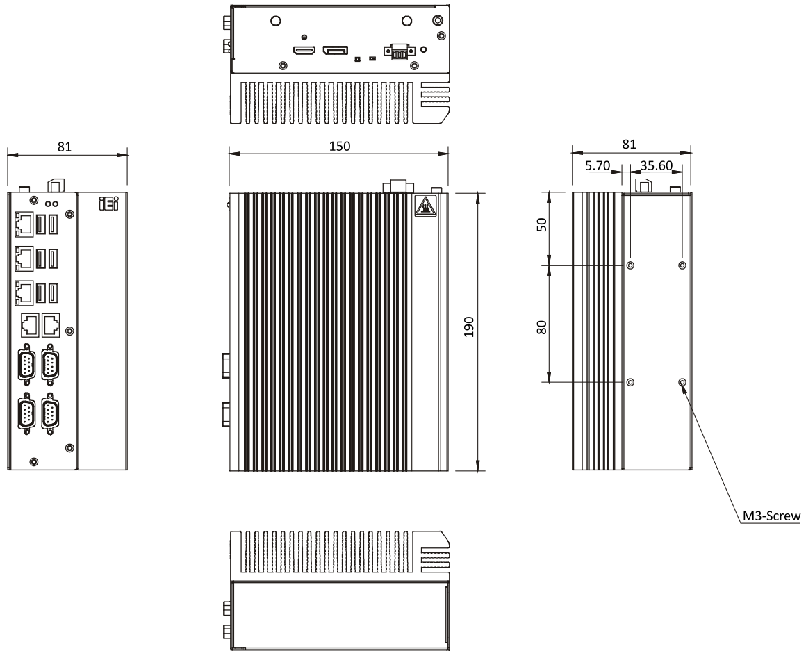
Figure 1-4: DRPC-230-ULT5-i5/8G/S Dimensions (mm)
