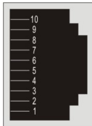
10-pin RJ-45
