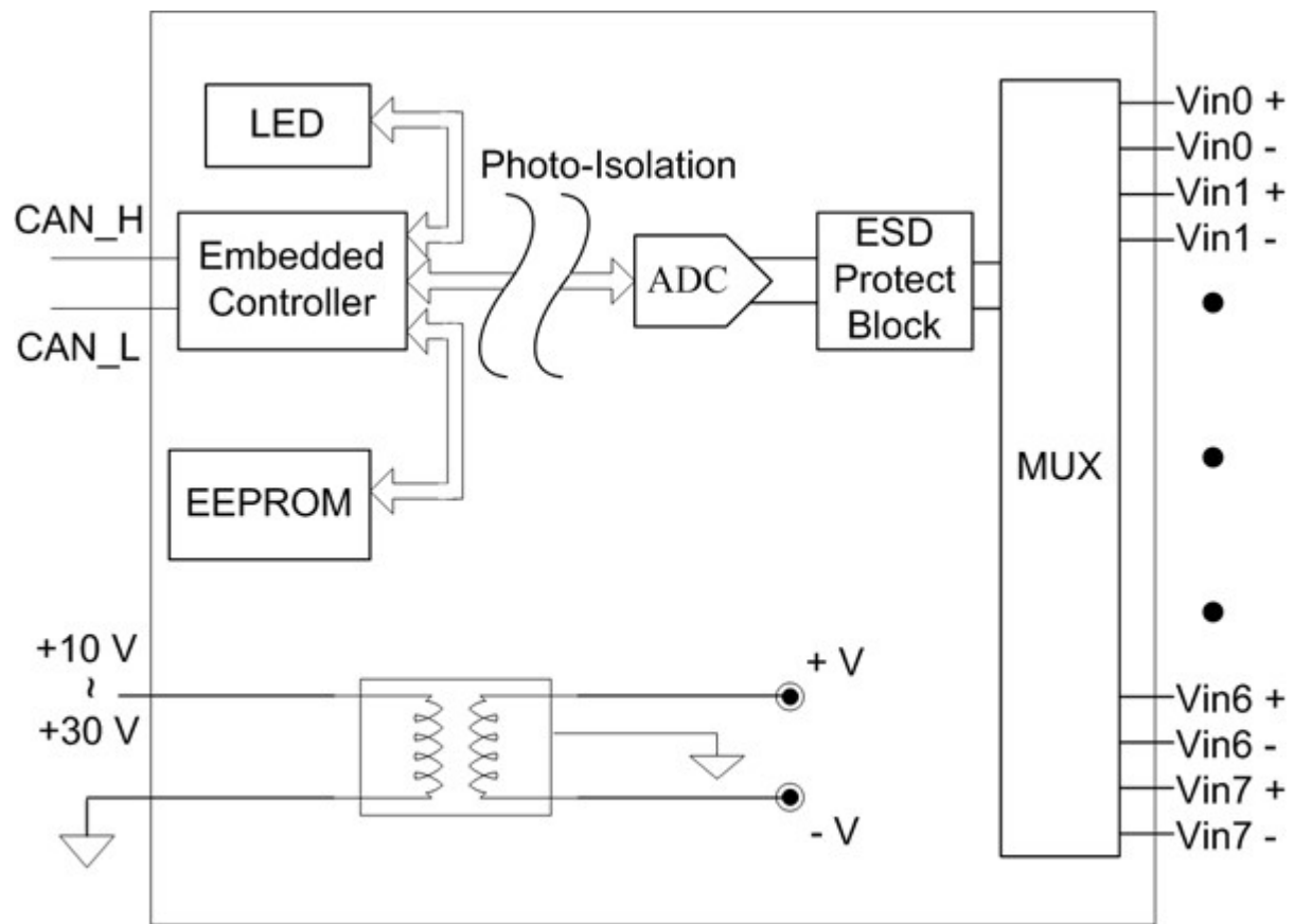
CAN-2017 Internal I/O Structure
