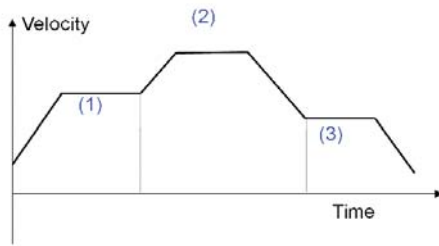
Multi-Axis Continuous Interpolation (With Acc. and Dec.)
