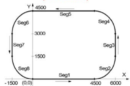
Continuous interpolation
