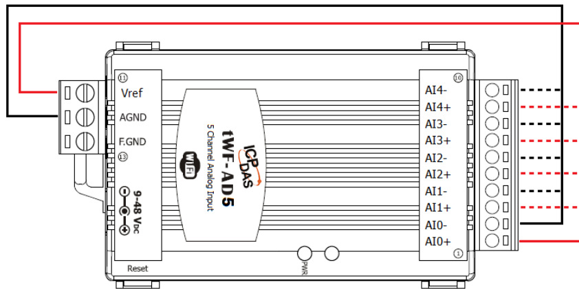
Figure 3-1: tWF-AD5 self-calibration wiring
