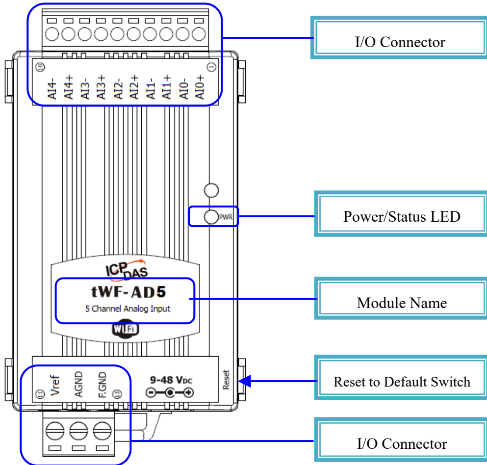
Figure 2-1: Front Panel of the tWF-AD5 module
