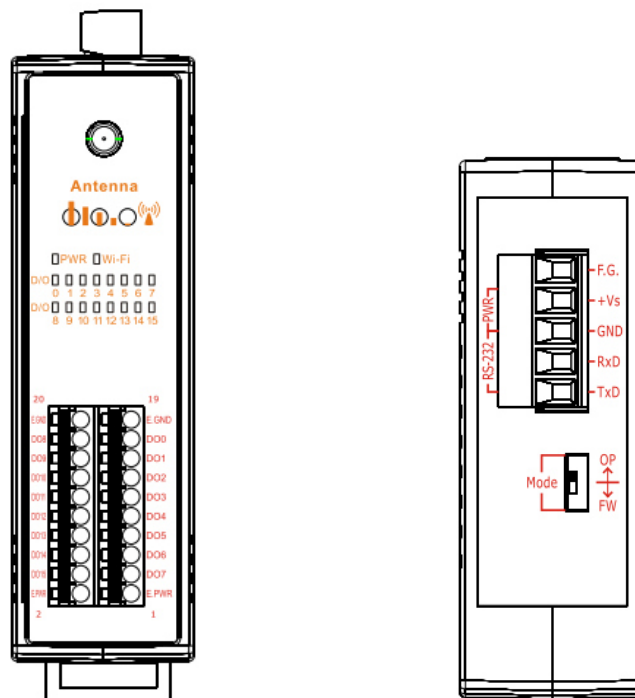
Figure 1: Appearance of the WF-2042
