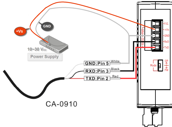
Figure 4: Power and Serial port wire connection
