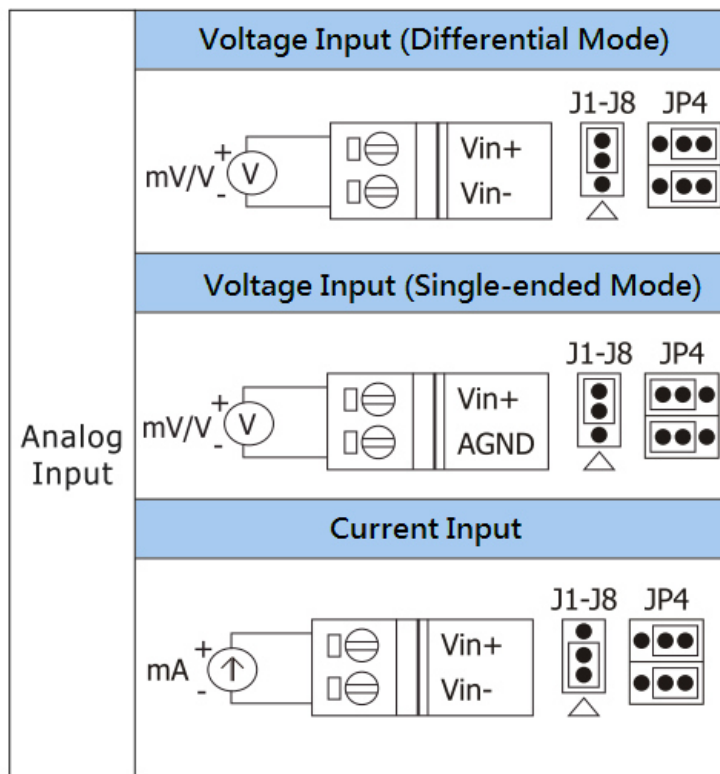
Figure 4: Wire connections
