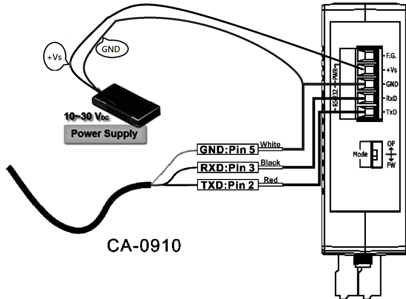
Figure 3: Power and Serial port wire connection
