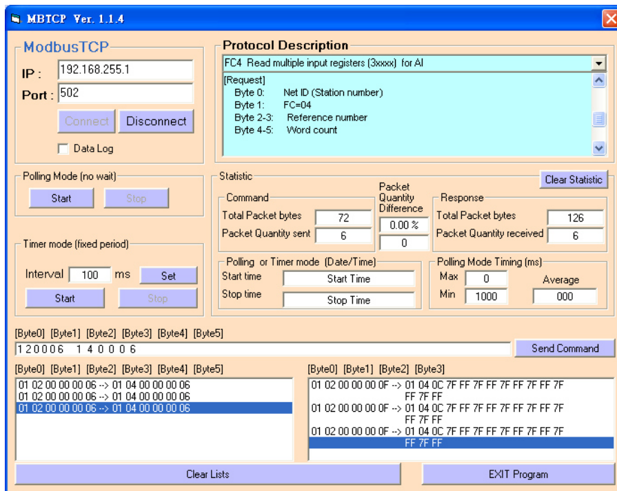
Figure 9: Read multiple input registers for AI
