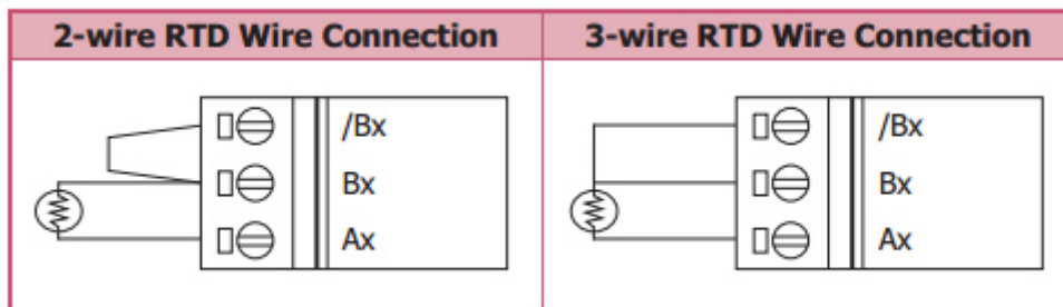
Figure 5: RTD wire connection
