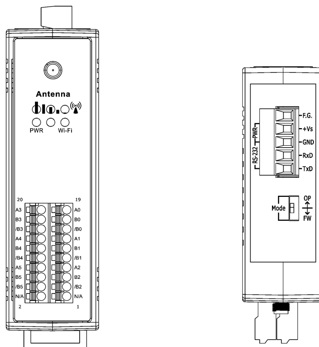
Figure 1: Appearance of the WF-2015
