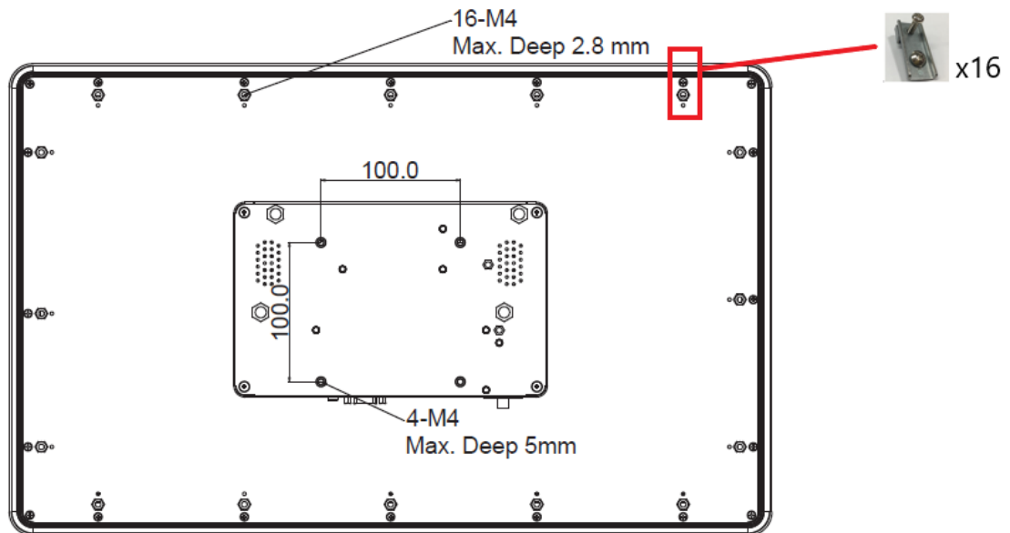
▲ P6217W-V3 Panel Mount kits
