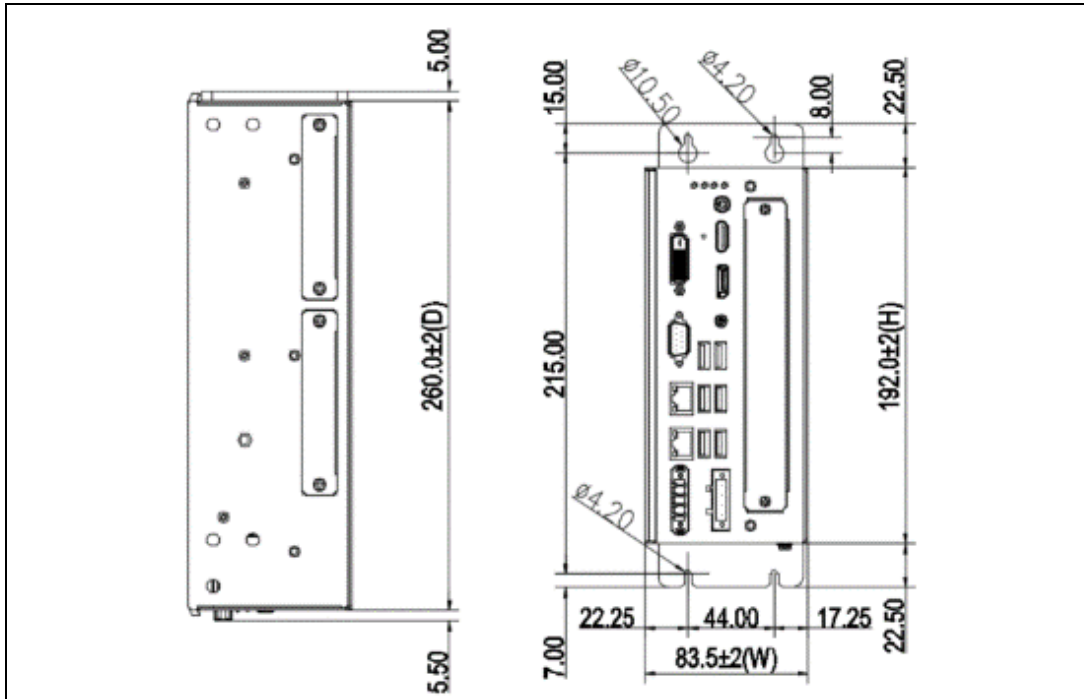
System w/ wall mount kit
