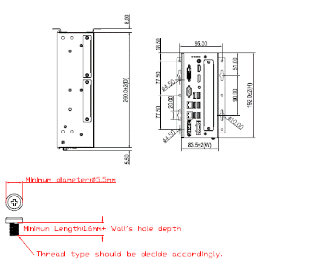
System w/ wall mount kit
