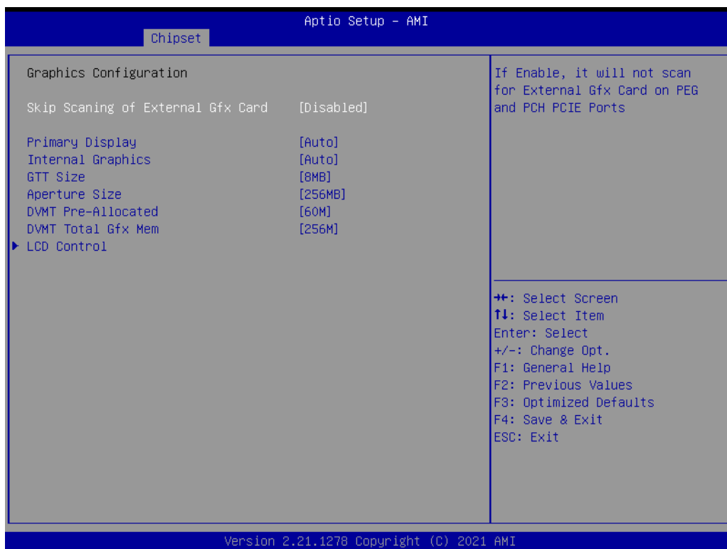
Figure 3.37 Graphics Configuration
