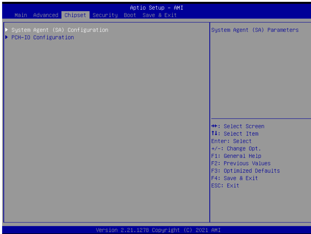
Figure 3.34 Chipset Setup
