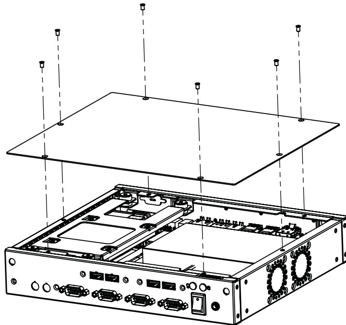
Figure 2.6 Close the Chassis Cover/ 盖上机箱顶盖 / 蓋上機箱上蓋
