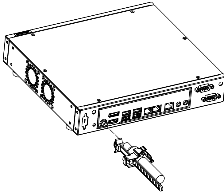
Figure 2.8 Installing the Snap Wire Bushing Lock harness/ 安装电源线防脱落扣具 / 安裝電源線防脫落扣具
