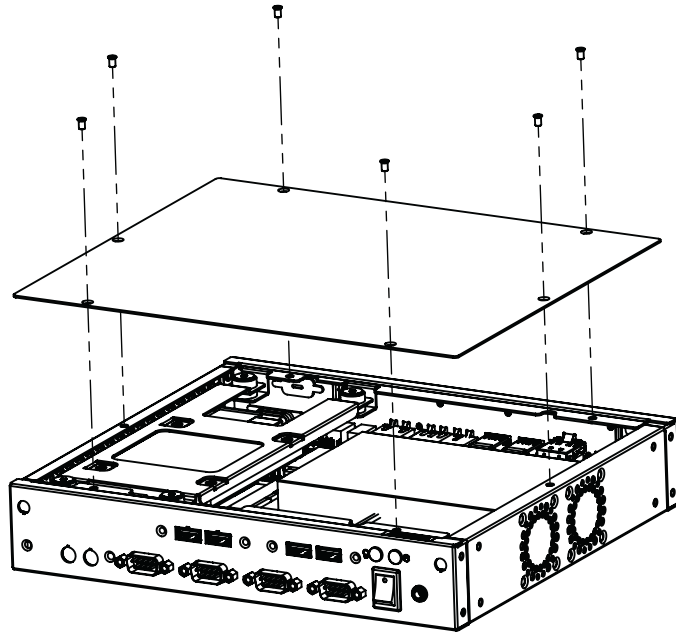
Figure 2.1 Open the Chassis Cover / 打开机箱顶盖 / 打開機箱上蓋
