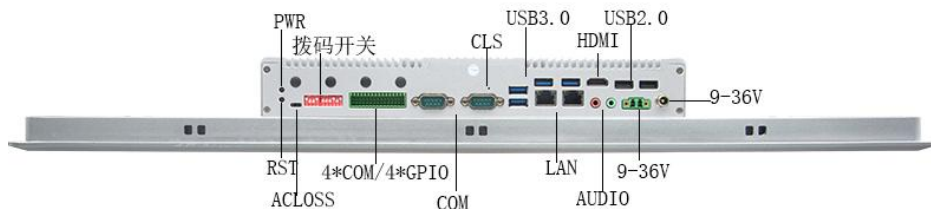
Image 3: P2381Y-C6 Bottom I/O View
