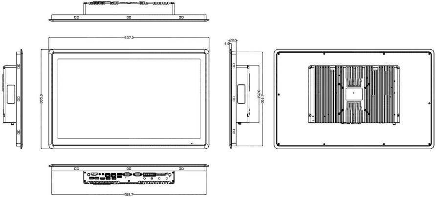
P2181Y-C6 Dimension
