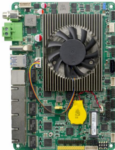
EPIC-W81P4 VER0.1 Front View
