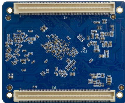
CK35 VER:1.0 Rear I/O View
