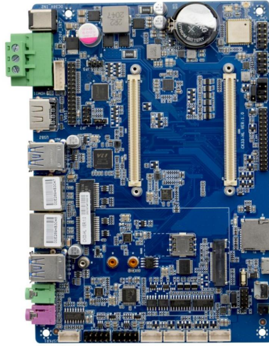
CK33-HL VER 1.0 Front View
