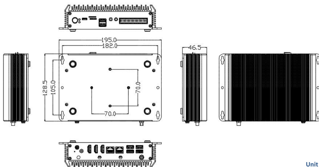
Unit: MM
