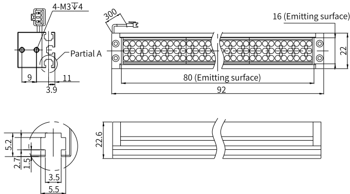
Partial A M3 nut slot, for mounting
