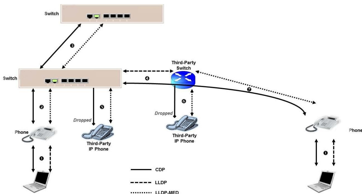
Figure CDP Operations
