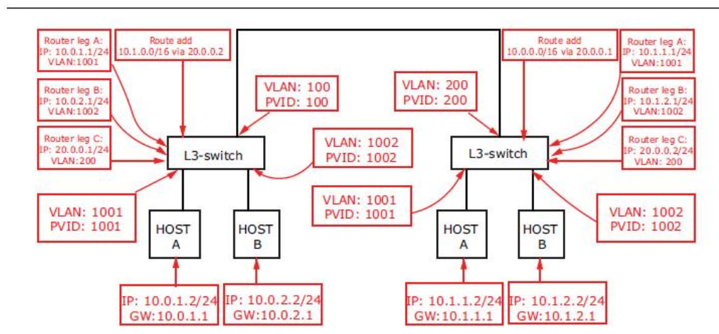
Figure • IPv4 Static Route
