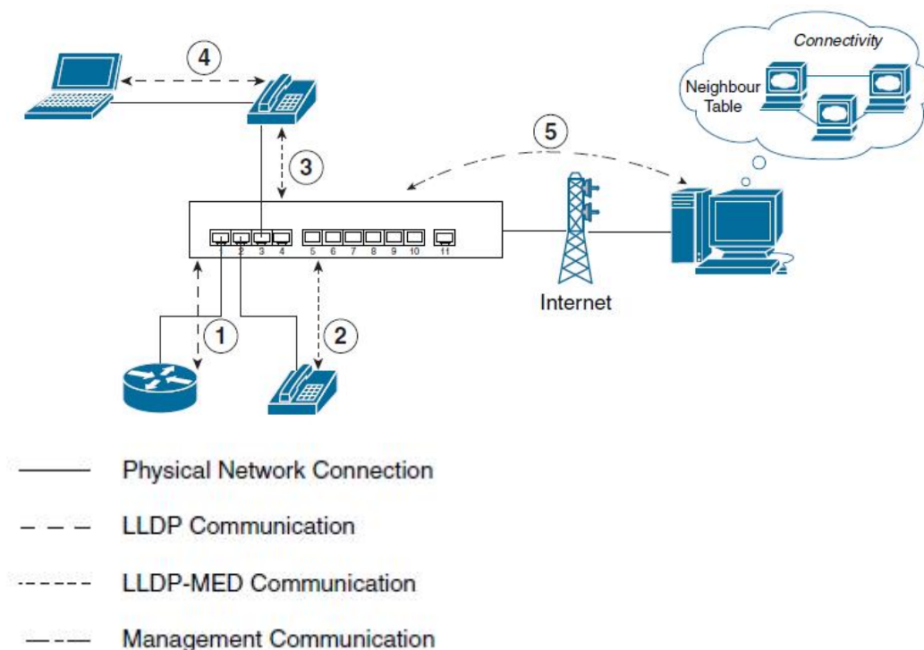
Figure LLDP Operations
