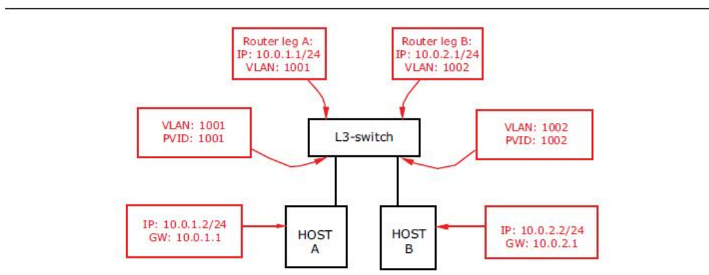
Figure • IP Routing using a Router and L3 Switch
