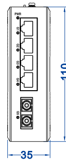
IES2305-4GT1GF-P48, IES2305-4GT1GF-P220
