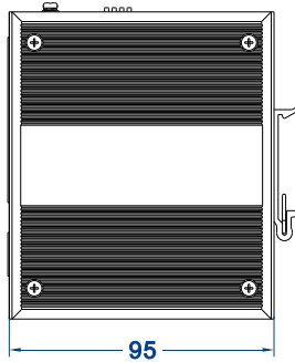
IES2305-4GP1GF-P48
