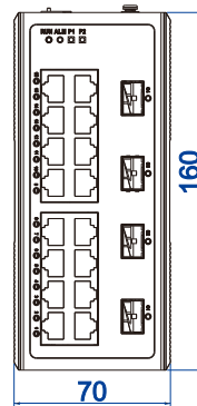
IES2220-16T4GS-2P48
