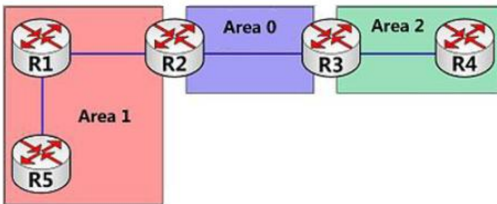
Figure 239 Area Partition
