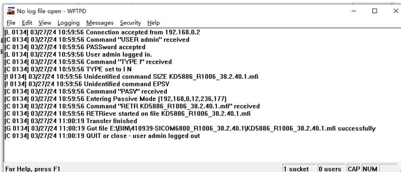
Figure 32 Normal Communication between FTP Server and Switch
