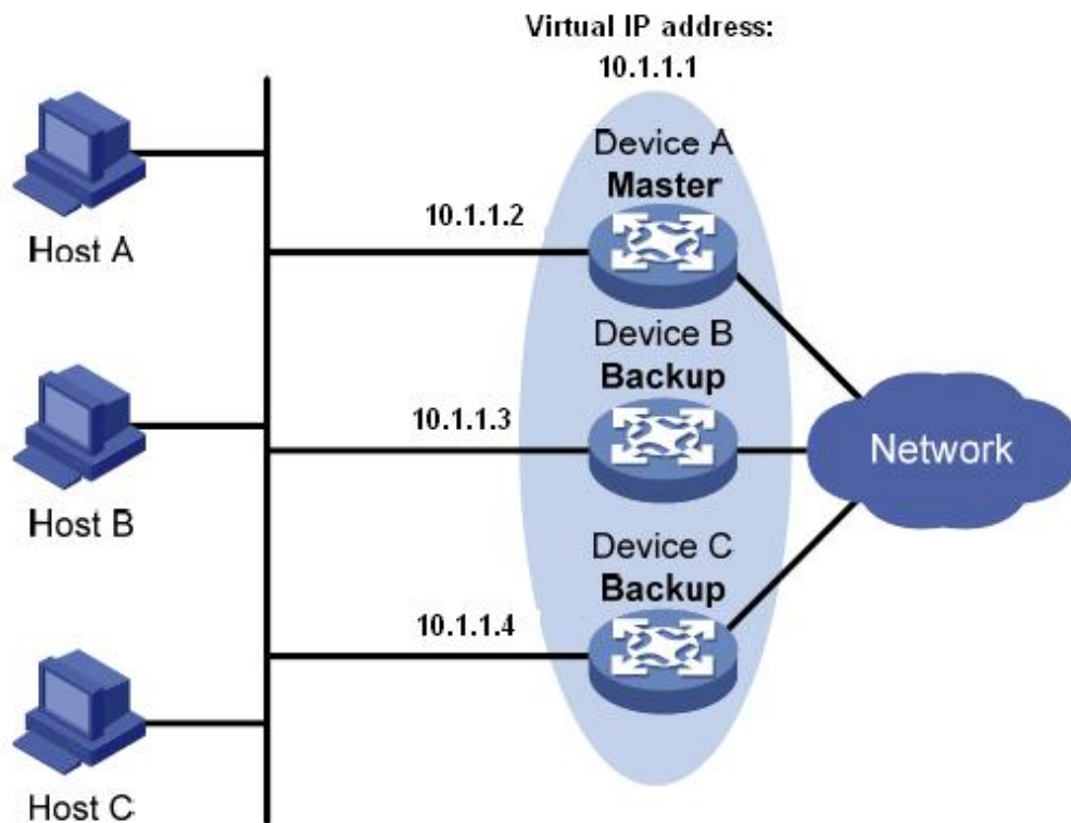
Figure 266 VRRP
