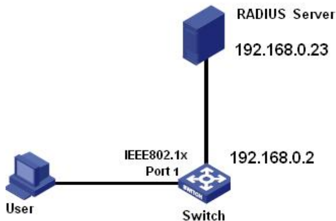
Figure 71 RADIUS Authentication Configuration Example
