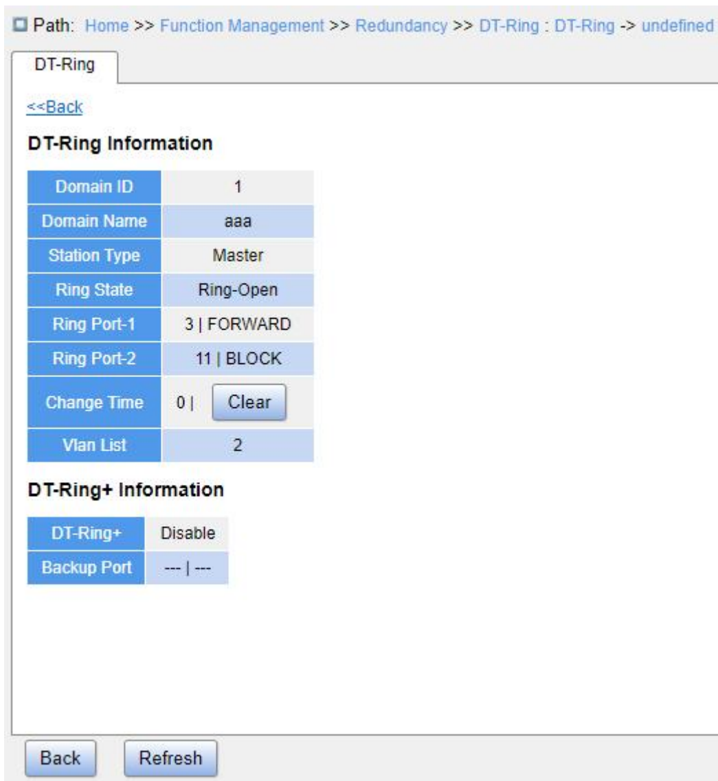
Figure 126 DT-Ring State
