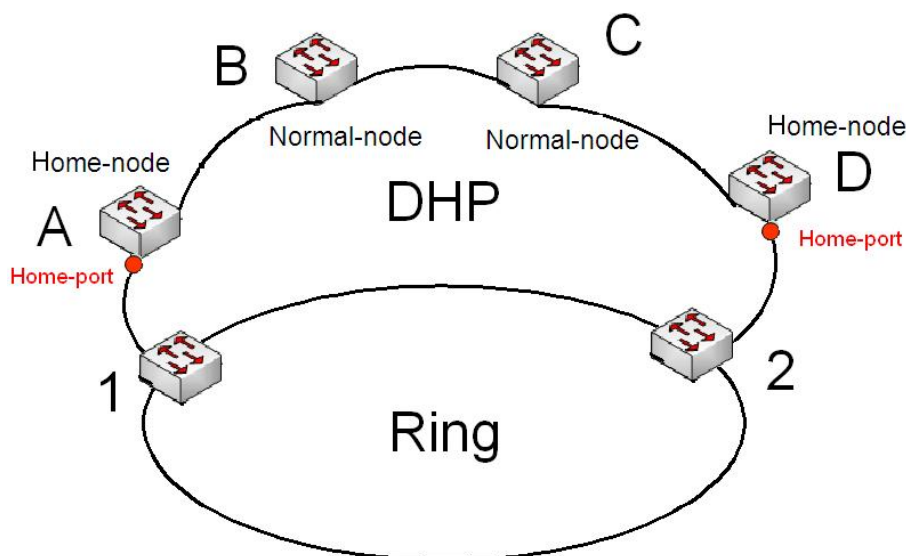
Figure 130 DHP Application
