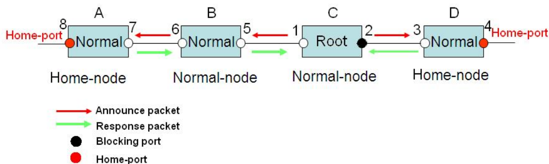
Figure 131 DHP Configuration
