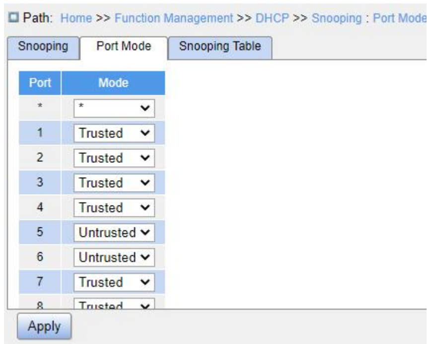
Figure 190 Configure Trust Port
