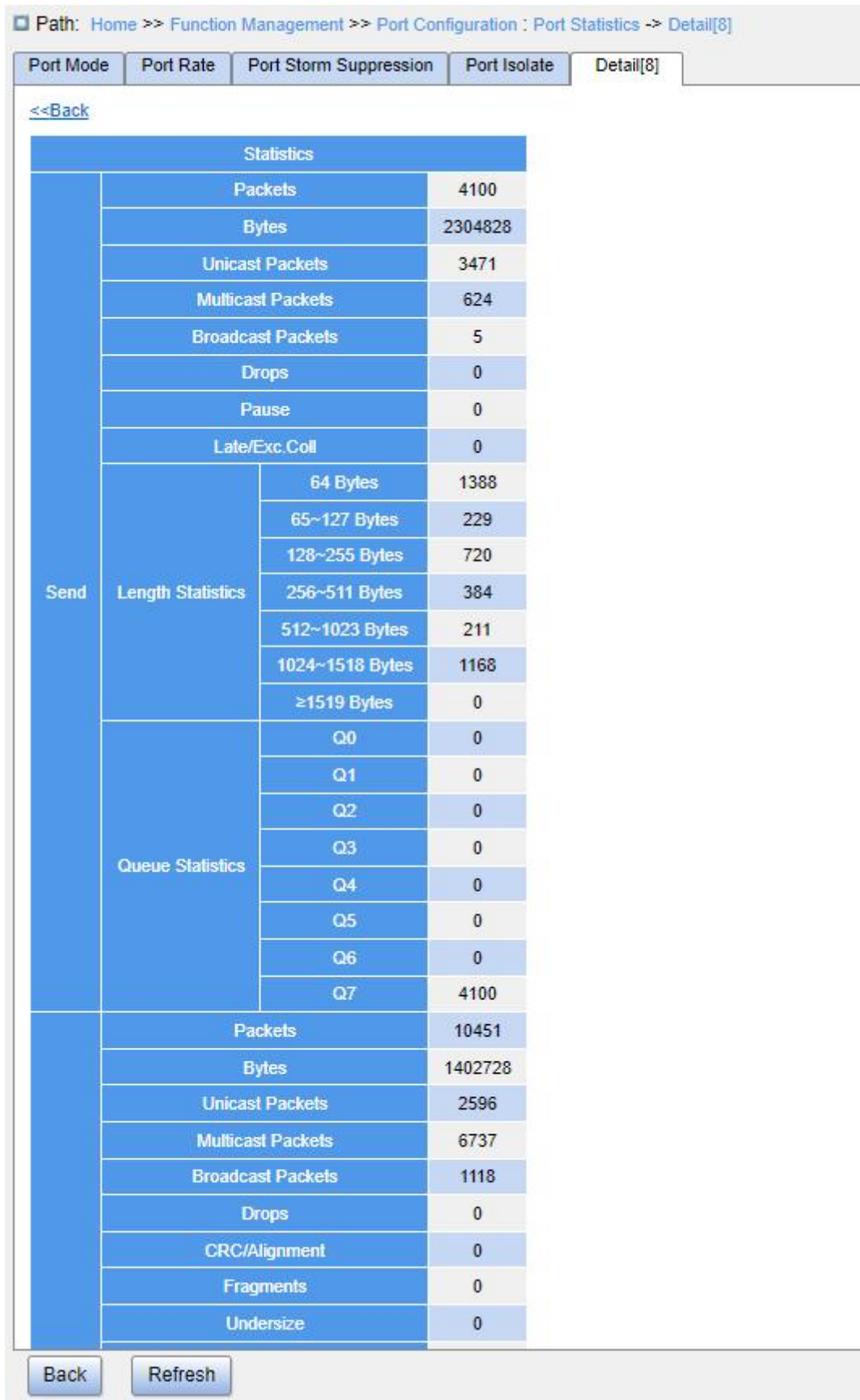
Figure 94 Port Detail Information Statistics
