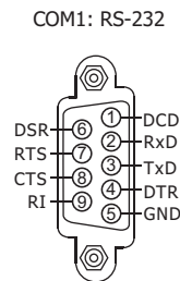
VH-23A1/25A1 COM Port
