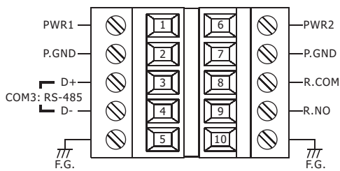
XP-8x47-CE6 Terminal Block
