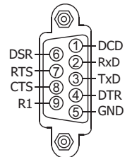
COM4: RS-232
