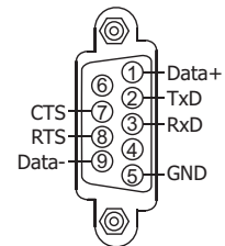
XP-8341-CE6/XP-8741-CE6 COM Port
