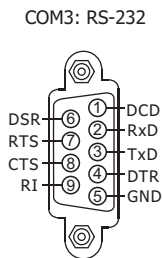
VP-23A1/25A1 COM Port
