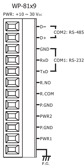
Terminal Block
