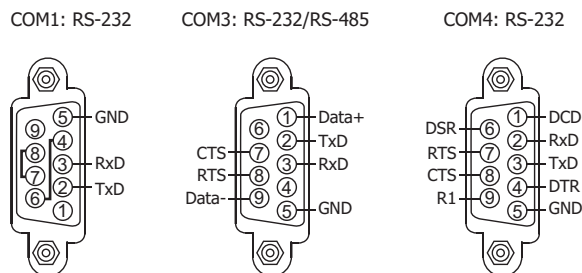
WP-84x9/88x9 COM Port
