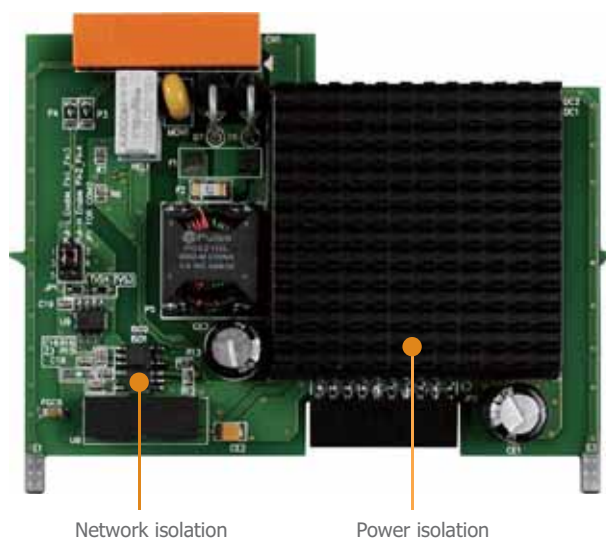
Network isolation
