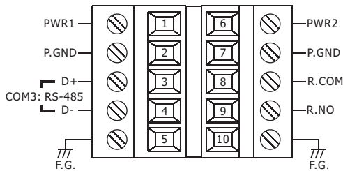
XP-8x41-Atom Terminal Block
