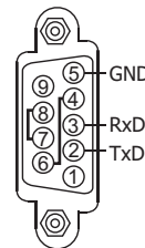
XP-8341-CE6/XP-8741-CE6 COM Port
