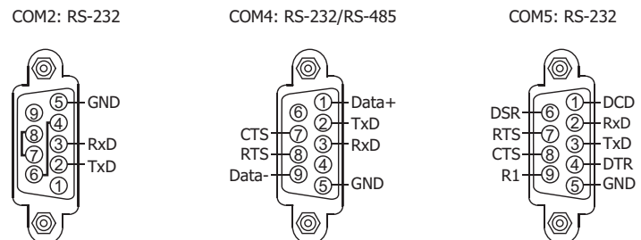
XP-8141-Atom-CE6/XP-8341-Atom-CE6/8741-Atom-CE6 COM Port
